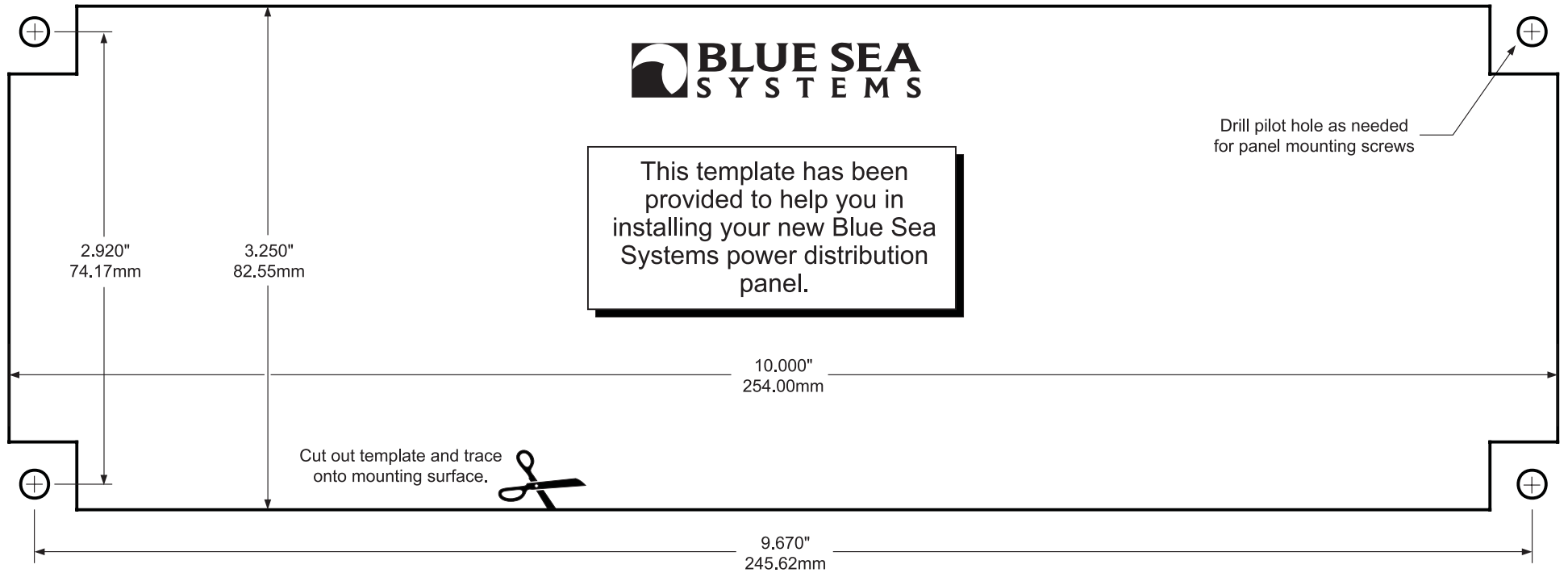
Horizontal 6 Position Panel Template
