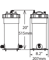
Pre-Filter Assembly
