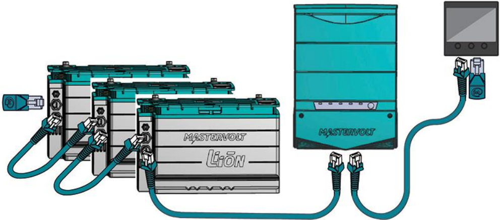
Figure 5: MasterBus cables
