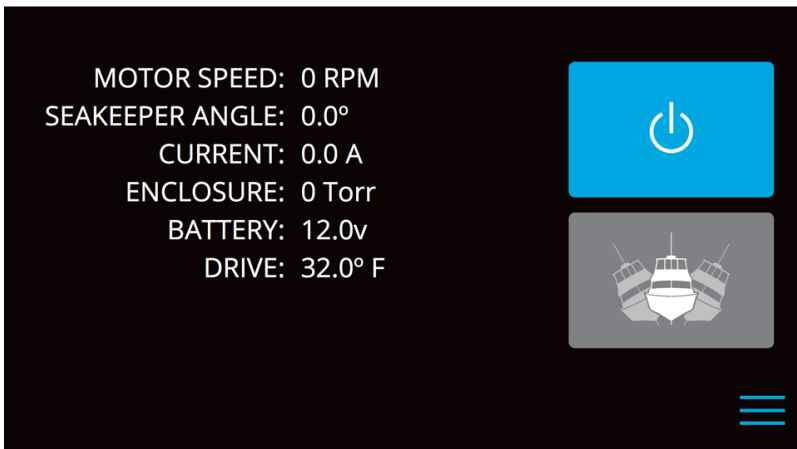
Figure 9: Service Page
