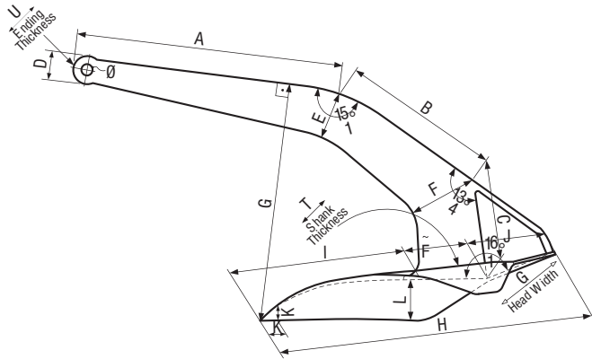
general dimensions
