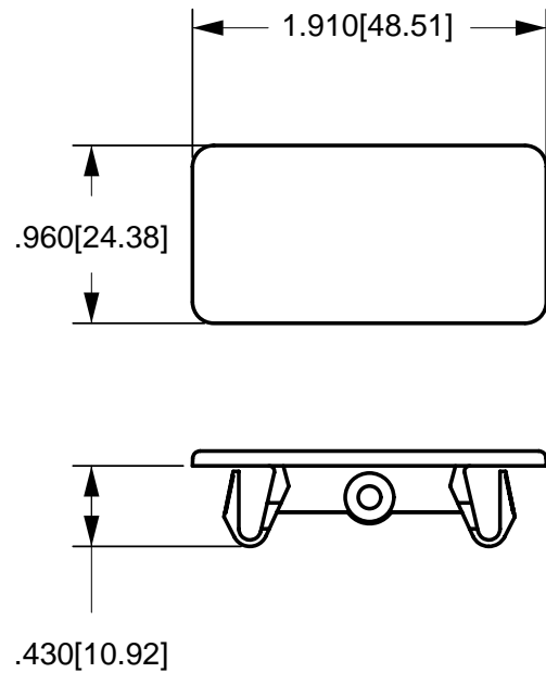
VHP MOUNTING PANEL PLUG Mastervolt part # 70906330
