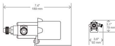
Booster Pump
