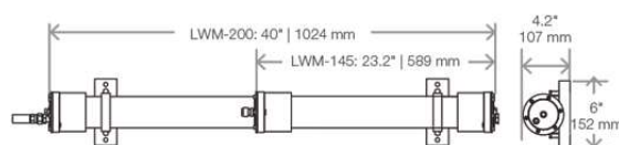
Membrane Assembly
