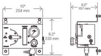
System Manifold
