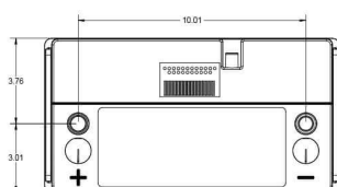
ODP-AGM31A LEFT POSITIVE SAE TERMINALS
