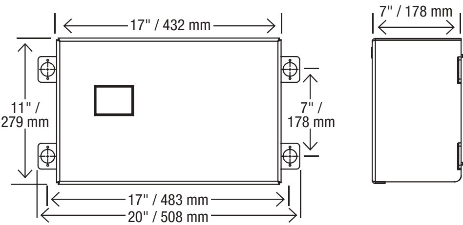
Control Panel - Front
