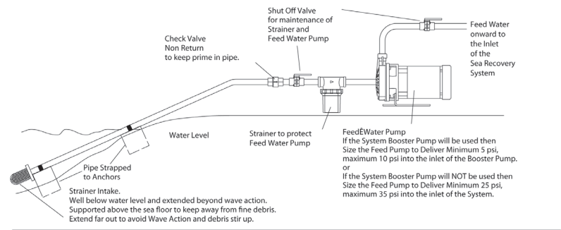
Example of Feed Water Intake from a Shallow Beach Well for a Land Installation.
